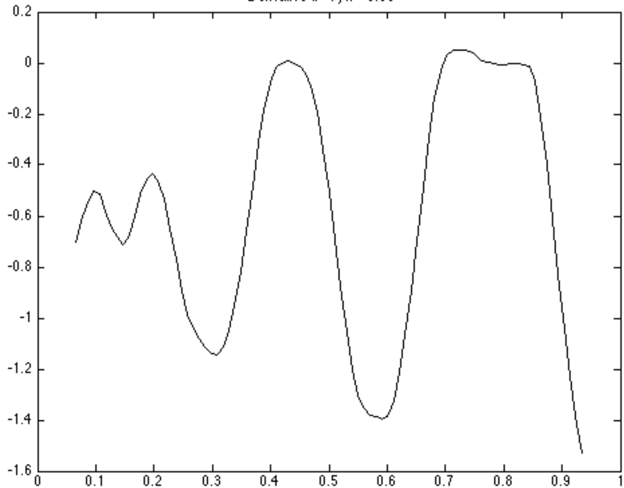
Derivative u = f' , h = 0.06
