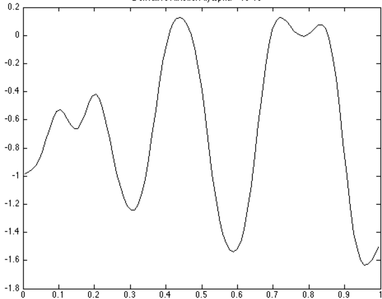
Derivative function u, alpha = 1e-10
