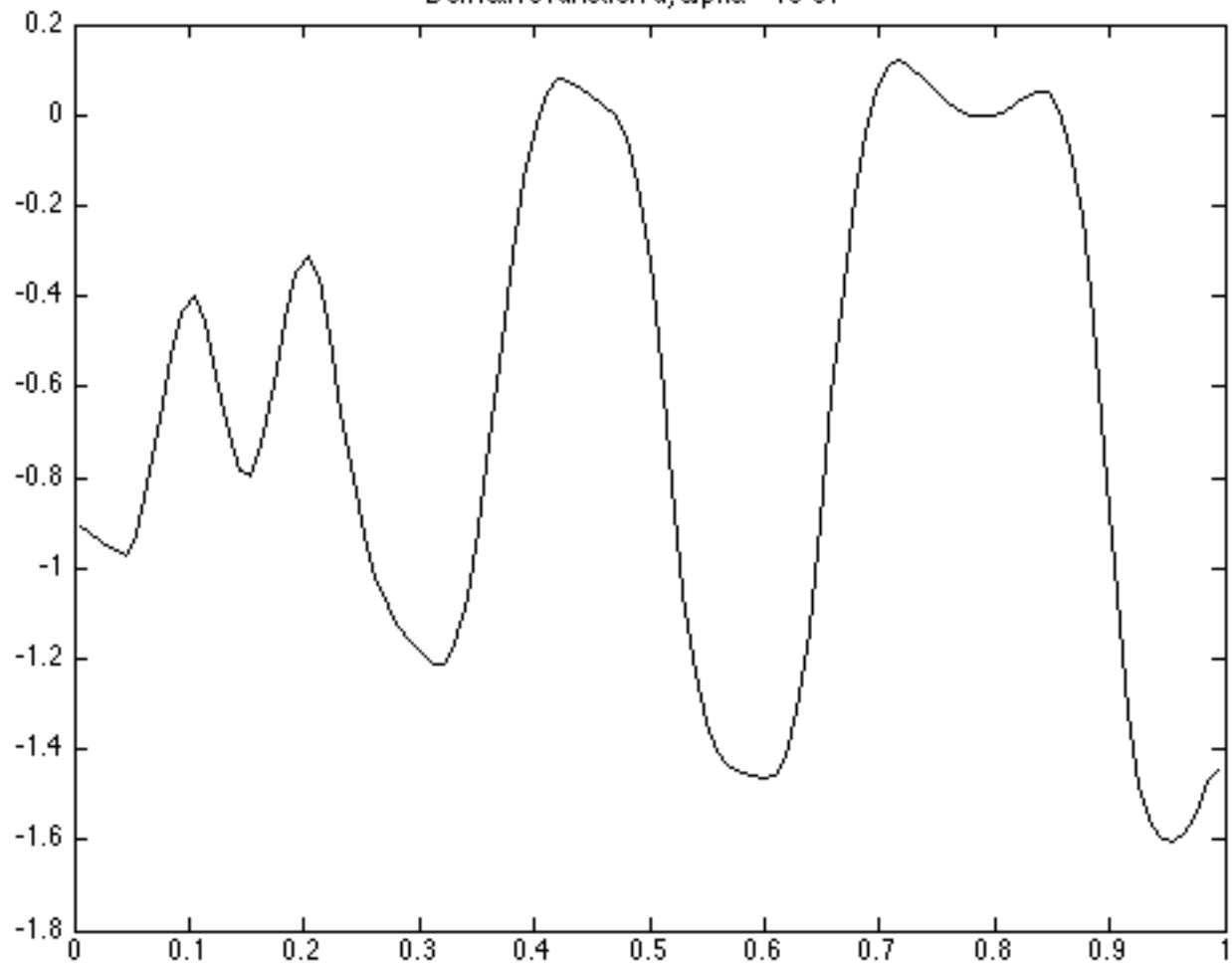
Derivative function u, alpha = 1e-07
