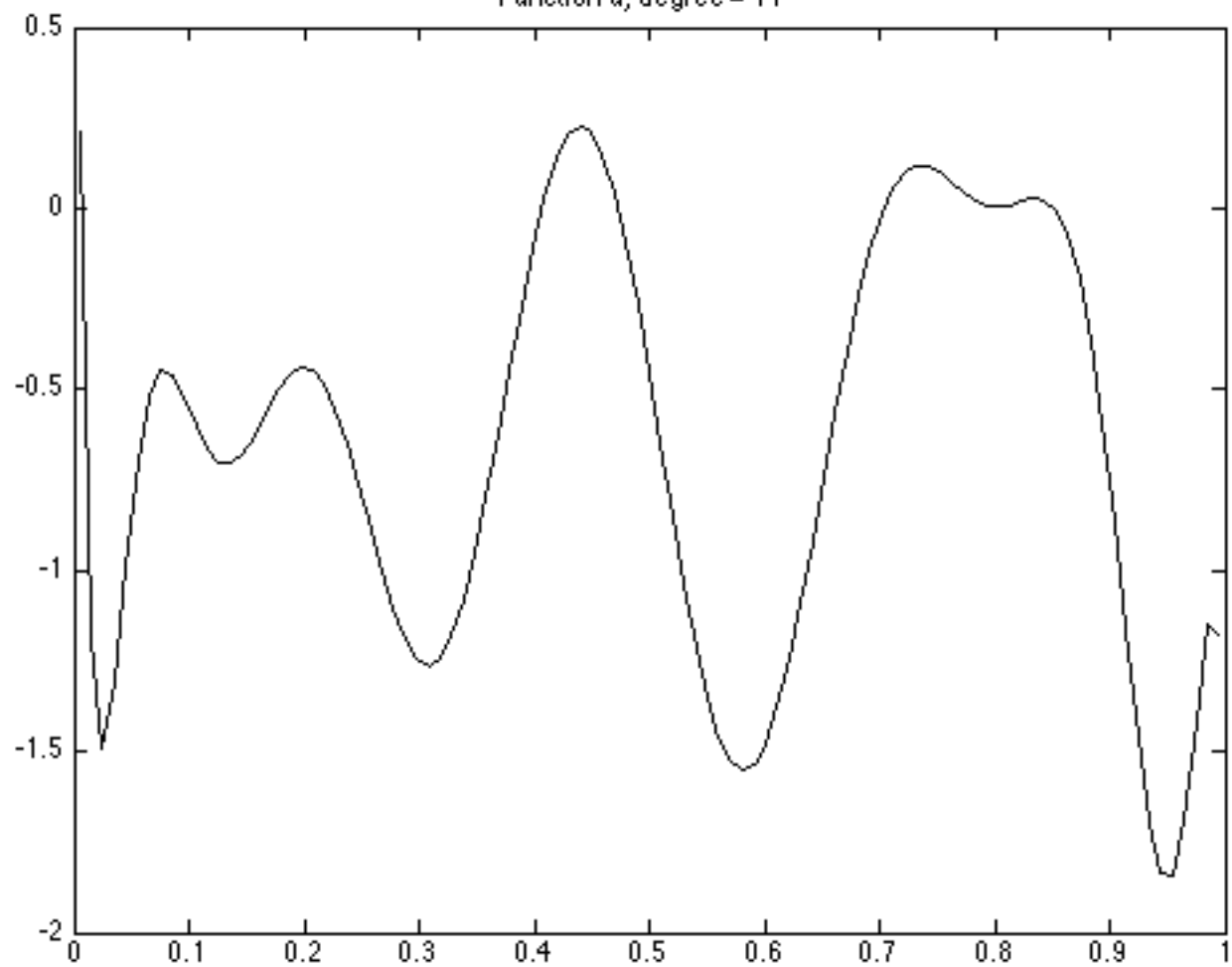
Function u, degree = 14
