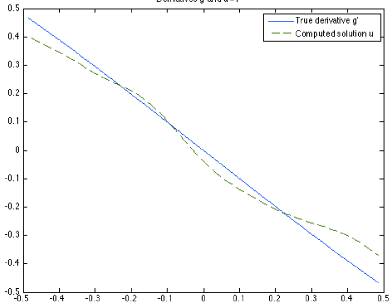
Derivatives g' and u = f'
