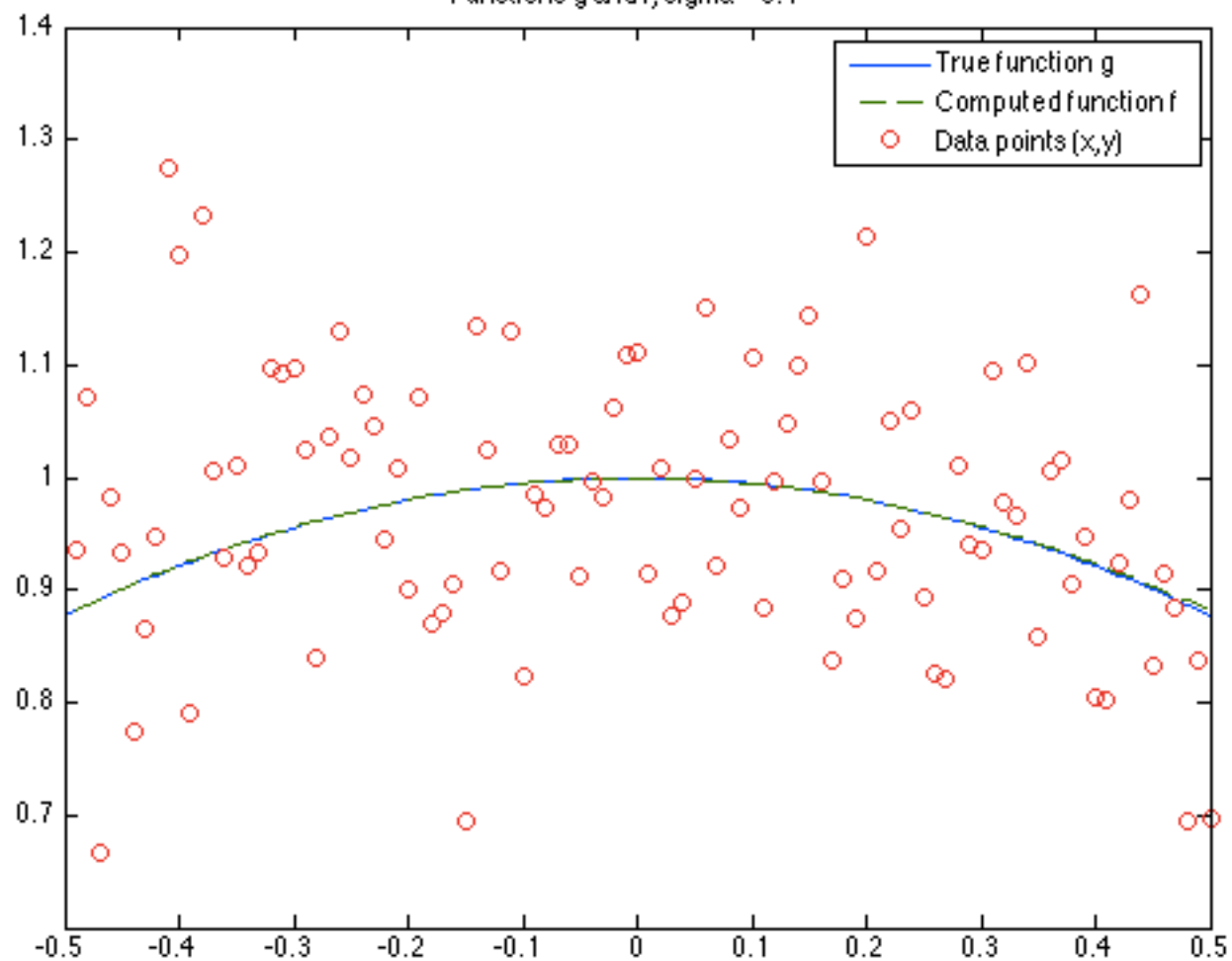
Functions g and f, sigma = 0.1
