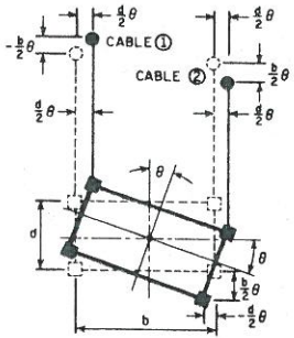
TORSIONAL DEFORMATION
