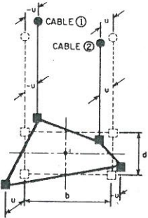
WARPING DEFORMATION
